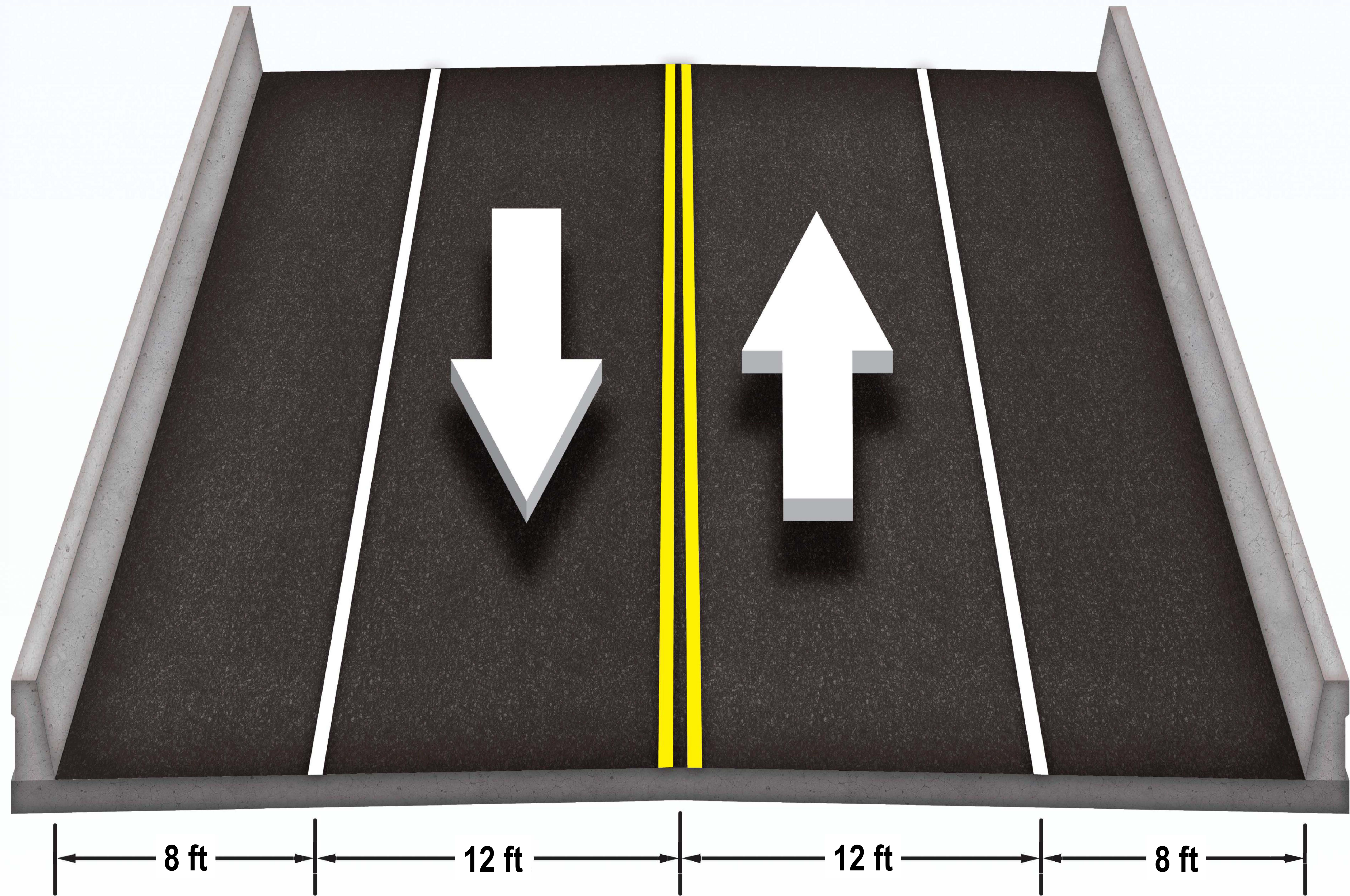
Proposed Bridge Typical Section CR 361 over Spring Warrior Creek Bridge Replacement
